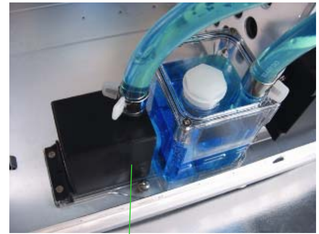
Pump & tank assembly
